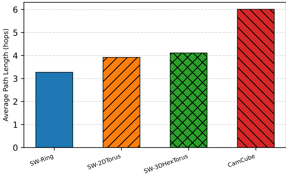
Fig. 3 — Dijkstra Average Path Length (N=512, degree-6)
